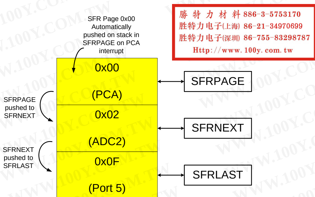
Figure 11.7. SFR Page Stack Upon PCA Interrupt Occurring During an ADC2 ISR
