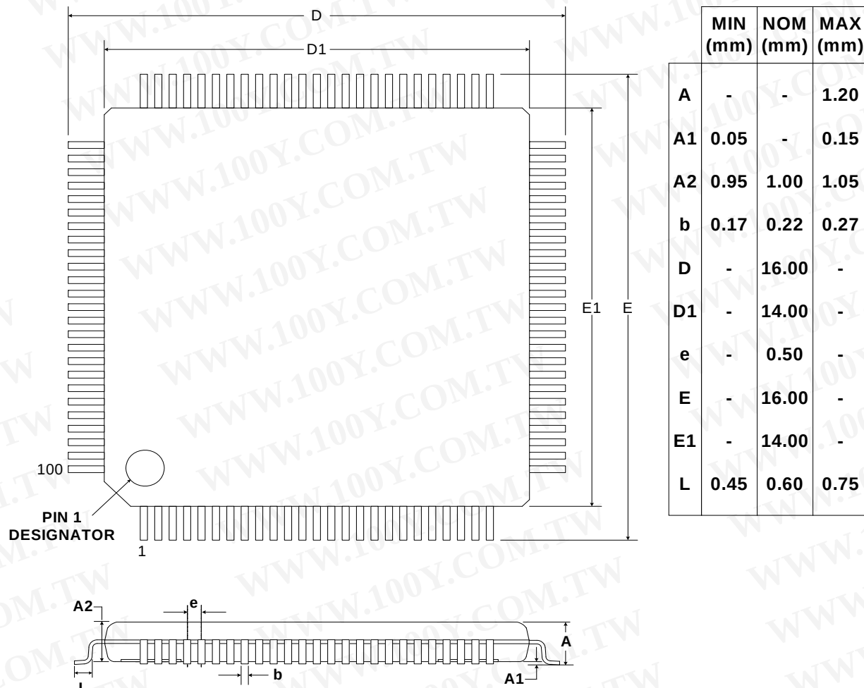
Figure 4.3. TQFP-100 Package Drawing
