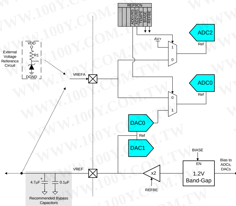
Figure 9.2. Voltage Reference Functional Block Diagram (C8051F121/3/5/7)
