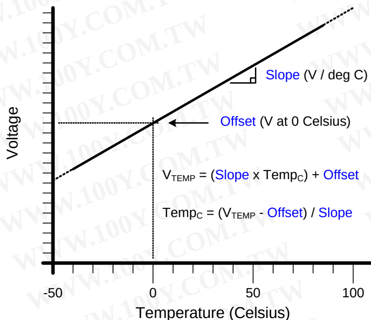
Figure 5.2. Typical Temperature Sensor Transfer Function
