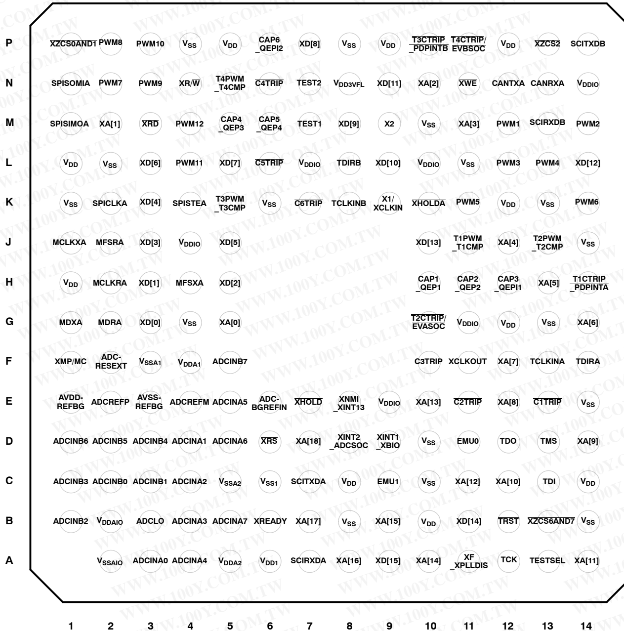
Figure 2-1. TMS320F2812 and TMS320C2812 179-Ball GHG MicroStar BGA™ (Bottom View)
