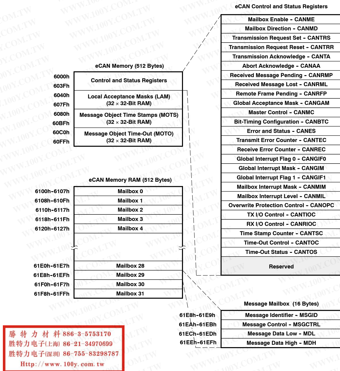
Figure 4-8. eCAN Memory Map
