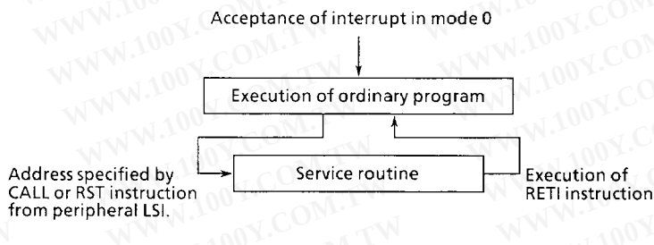
Figure 3.6 Interrupt Processing in Mode 0
