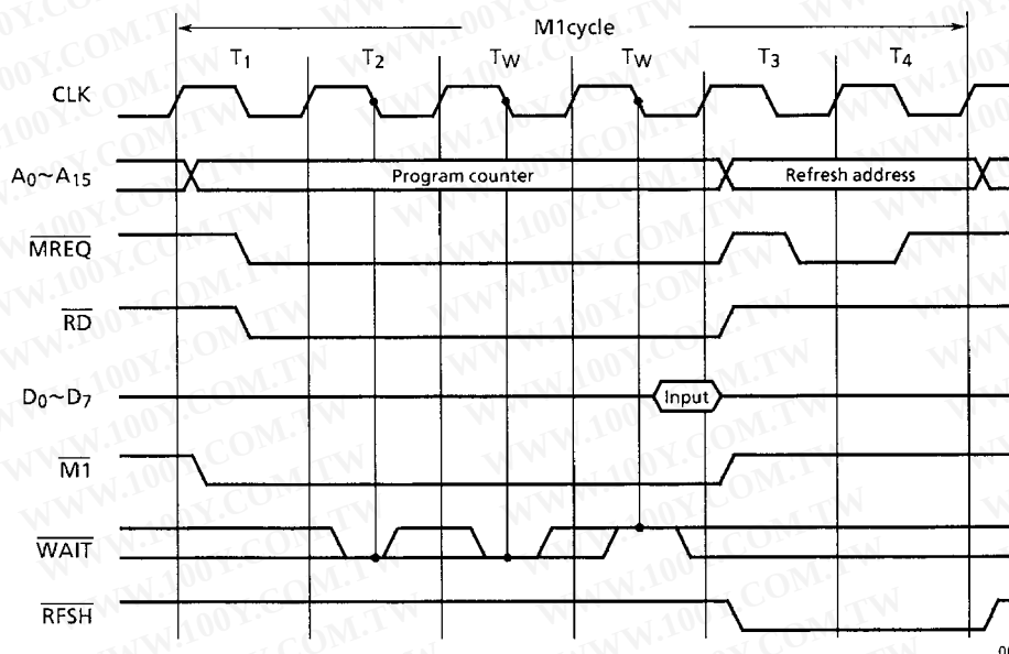
Figure 3.12 Opcode Fetch Timing Including Wait State
