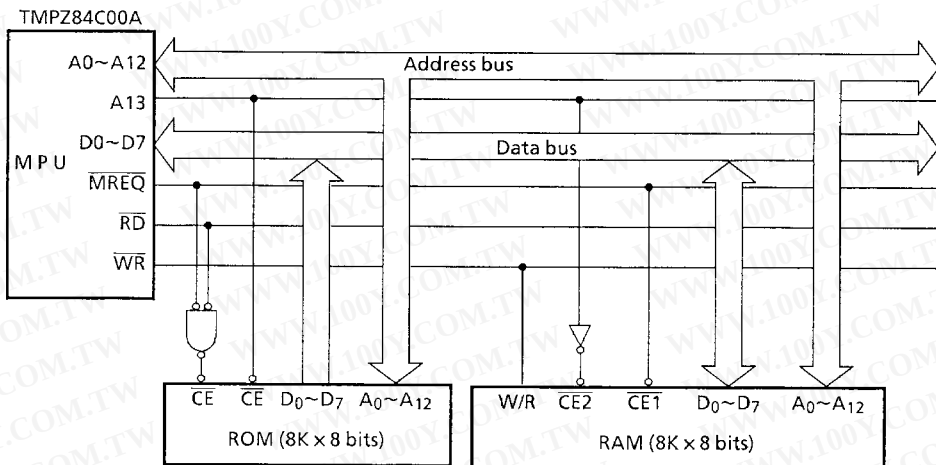
Figure 3.22 Example Connection with Memories
