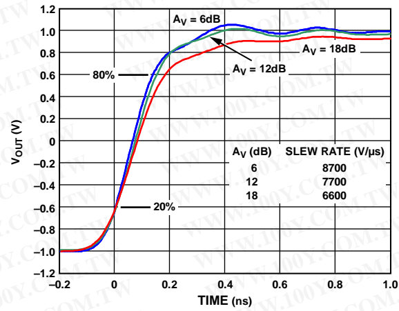
Figure 9. Rise Time, VOUT vs. Time, VOUT = 2 V p-p
