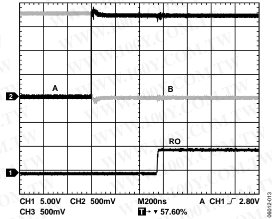
Figure 13. ADM483E Receiver t_{PLH}
