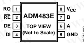
Figure 2. Pin Configuration
