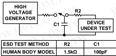
Figure 24. ESD Generator
