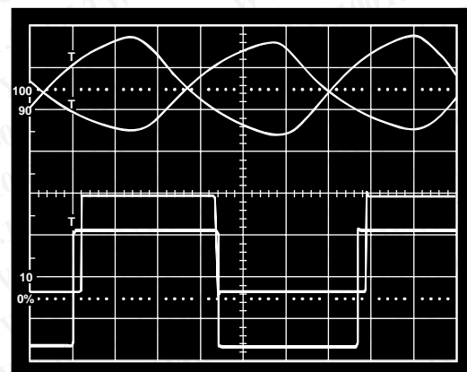
Figure 20. Driving 4000 Ft. of Cable
