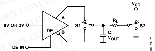
Figure 8. Driver Voltage Measurement Test Circuit 2
