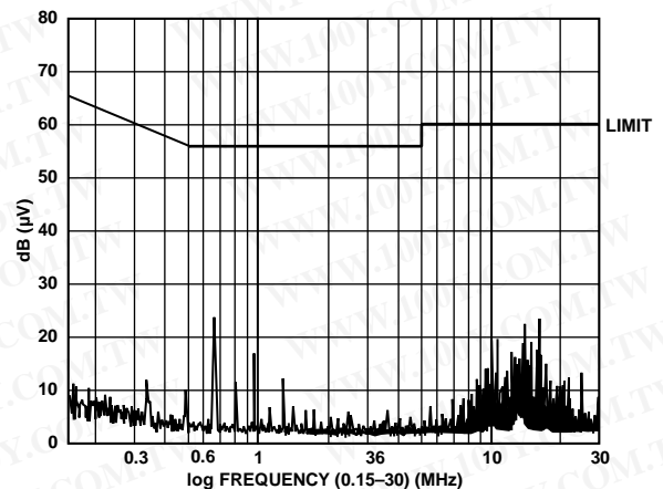
Figure 29. Conducted Emissions
