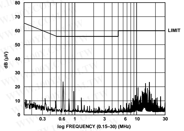
Figure 23. Conducted Emissions
