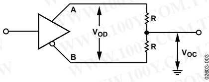
Figure 3. Driver Voltage Measurement
