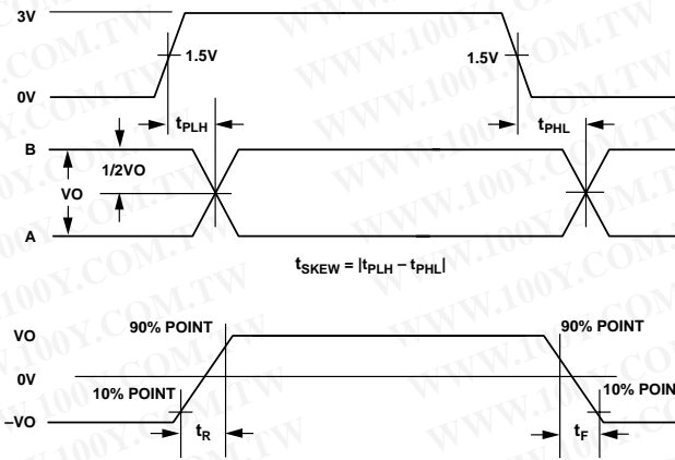
Figure 9. Driver Propagation Delay, Rise/Fall Timing
