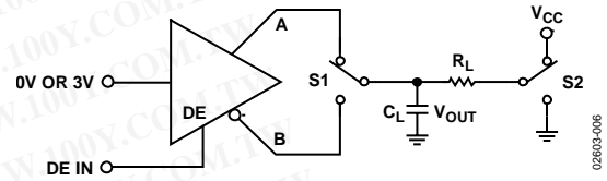
Figure 6. Driver Enable/Disable
