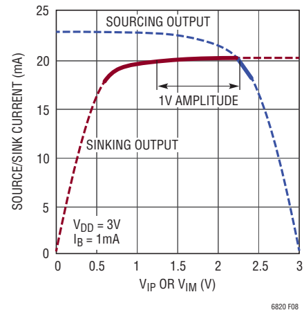
Figure 8. Drive Source/Sink vs Output Voltage
