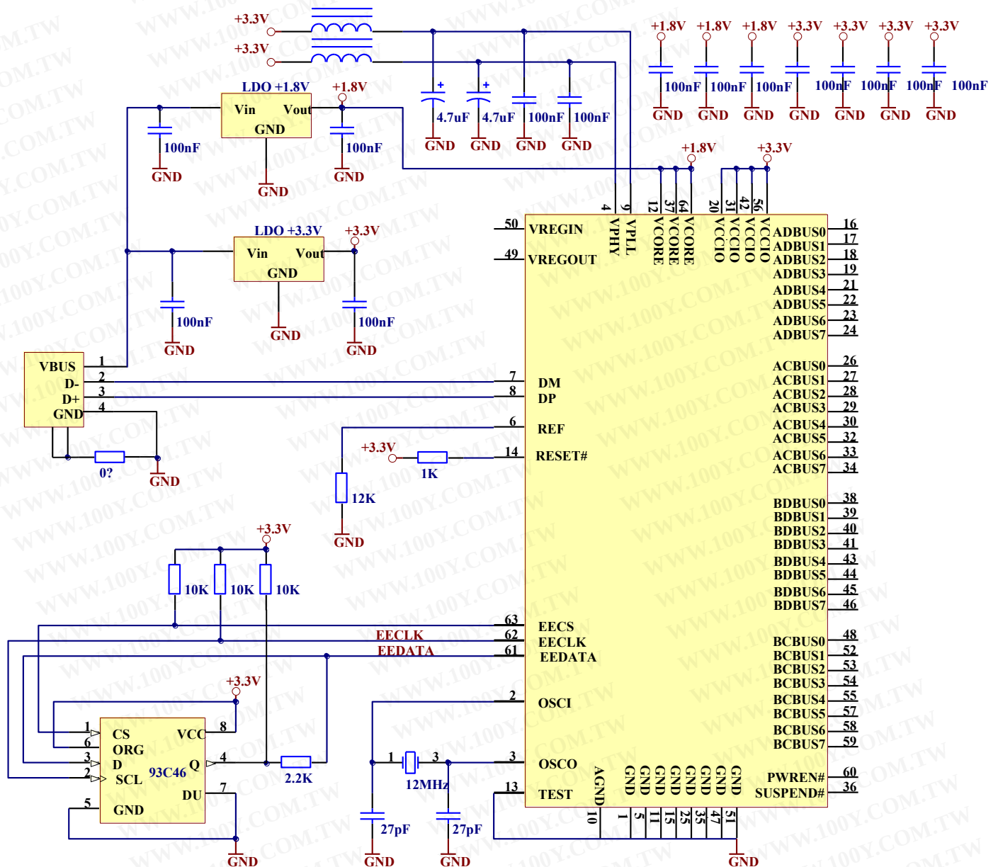
Bus Powered Application example 2: Bus powered configuration (with additional 1.8V LDO voltage regulator for VCORE)
