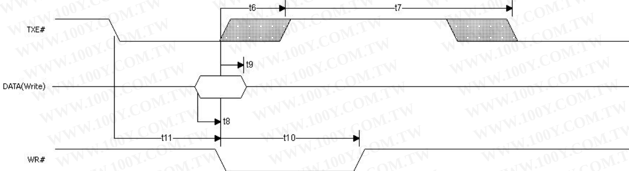
Figure 4.6 FT245 asynchronous FIFO Interface WRITE Signal Waveforms
