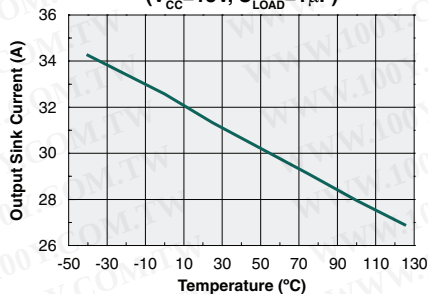
Output Sink Current vs. Temperature ( V_{CC}=18V , C_{LOAD}=1\mu F )
