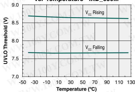
Under Voltage Lockout Threshold vs. Temperature - IXD_630M
