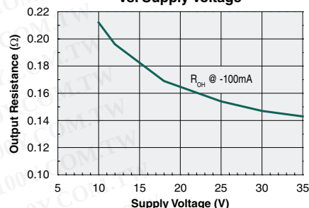
High-State Output Resistance vs. Supply Voltage
