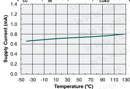
Dynamic Supply Current vs. Temperature ( V_{CC}=18V , V_{IN}=0-5V , f=1kHz , C_{LOAD}=5.6nF )
