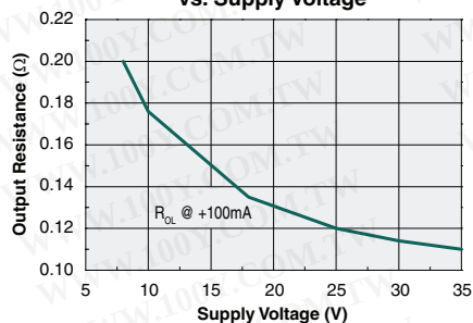
Low-State Output Resistance vs. Supply Voltage
