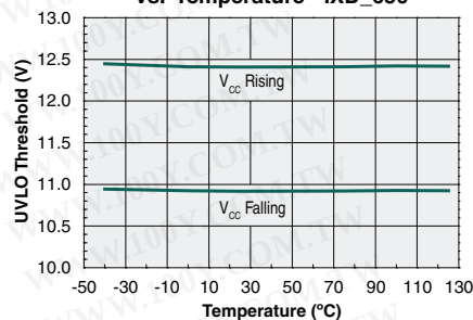
Under-Voltage Lockout Threshold vs. Temperature - IXD_630
