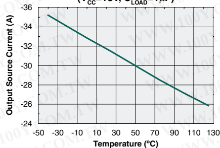
Output Source Current vs. Temperature ( V_{CC}=18V , C_{LOAD}=1\mu F )
