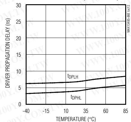
DRIVER PROPAGATION DELAY vs. TEMPERATURE (MAX13486E)
