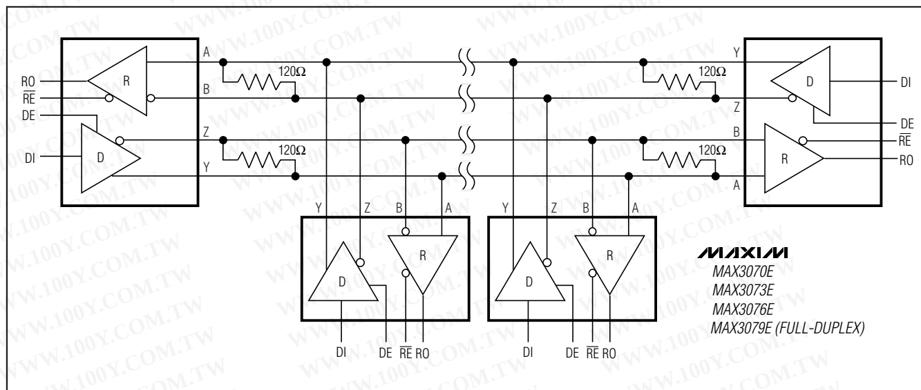
Figure 13. Typical Full-Duplex RS-485 Network
