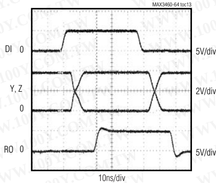
DRIVER AND RECEIVER PROPAGATION DELAYS
