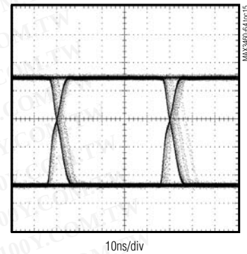
EYE DIAGRAM
