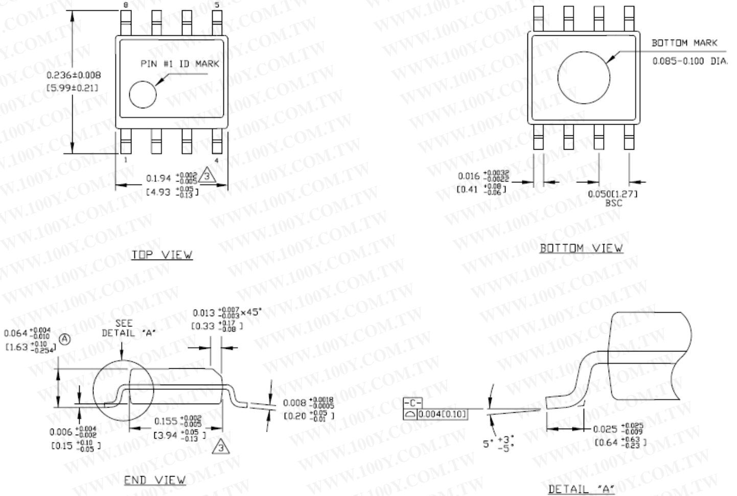
8-Pin SOIC
