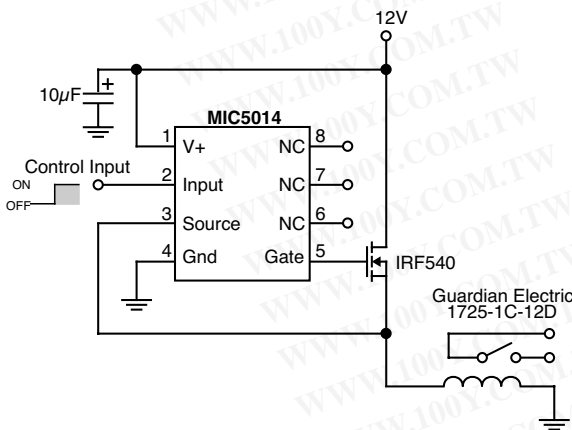
Figure 9: Relay Driver
