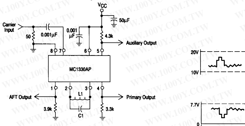
Figure 2. Test Fixture Circuit
