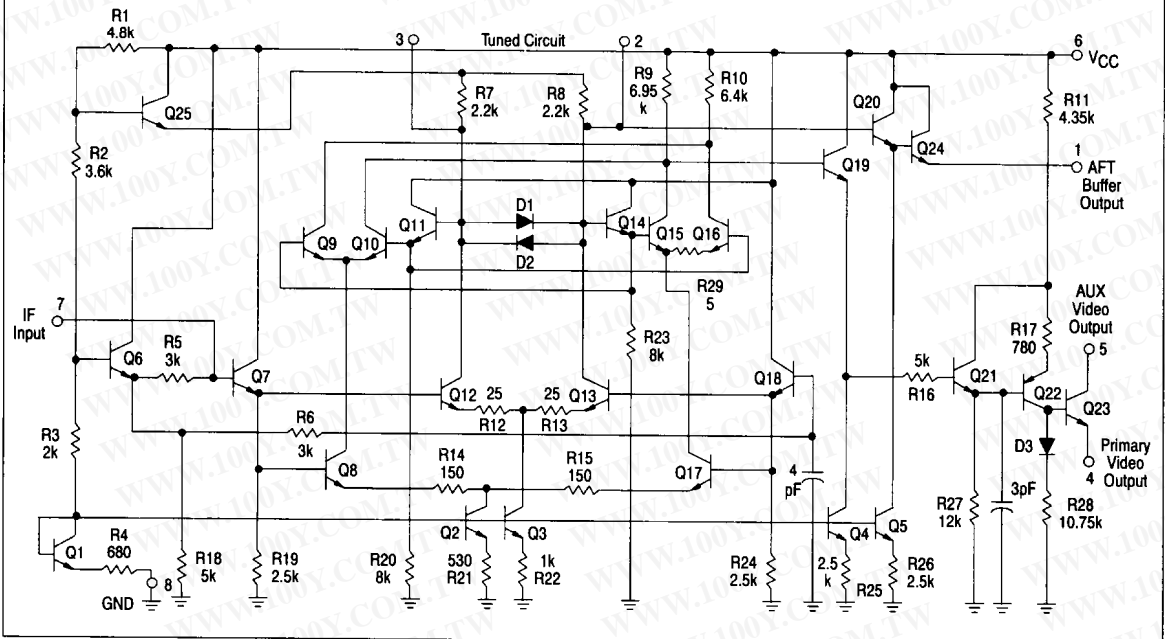
Figure 1. Circuit Schematic
