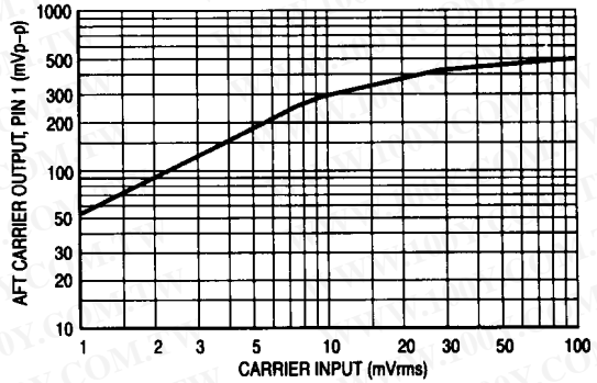
Figure 9. AFT Limiting
