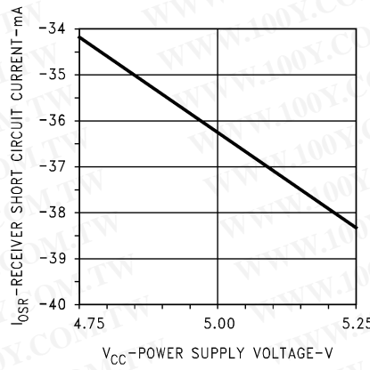
Receiver Short Circuit Current vs Power Supply
