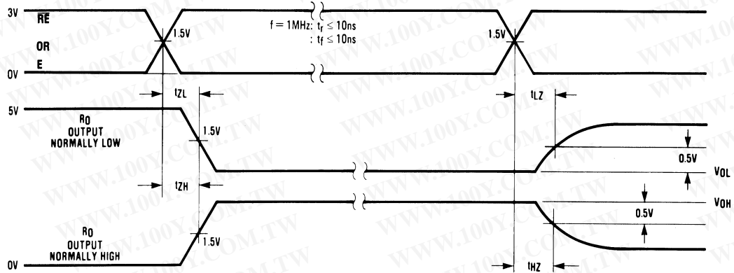
FIGURE 4. Receiver Enable/Disable Propagation Delay Timing
