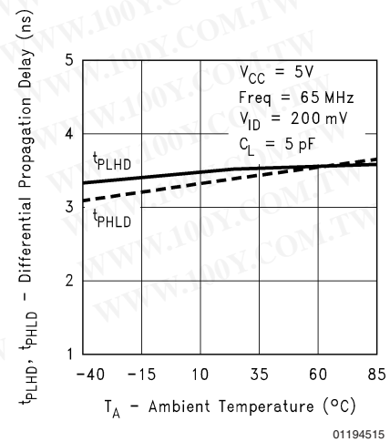
Differential Propagation Delay vs Ambient Temperature
