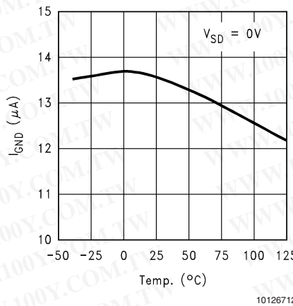
Ground Current Vs Temperature ( V_{SD} = 0V )
