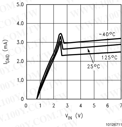
Ground Current Vs Temperature ( V_{SD} = V_{IN} )
