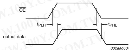
Fig 17. Output propagation delay
