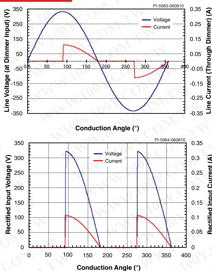
Figure 8. (a) Ideal Input Voltage and Current Waveforms for a Leading Edge TRIAC Dimmer at 90° Conduction Angle. (b) Resultant Waveforms Following Rectification of TRIAC Dimmer Output.
