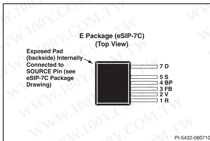
Figure 3. Pin Configuration.
