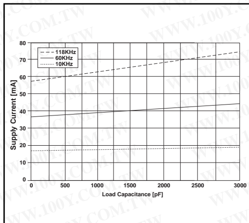
Figure 6. Supply Current VS. Load Capacitance when Transmitting Data for the SP3243E
