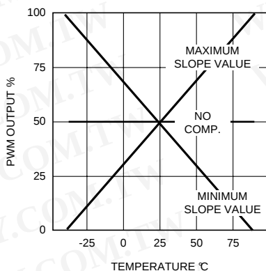
Figure 15. Temperature Compensation Principle
