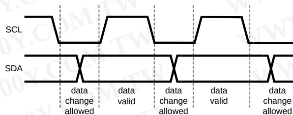
Figure 20. Data Validity Diagram
