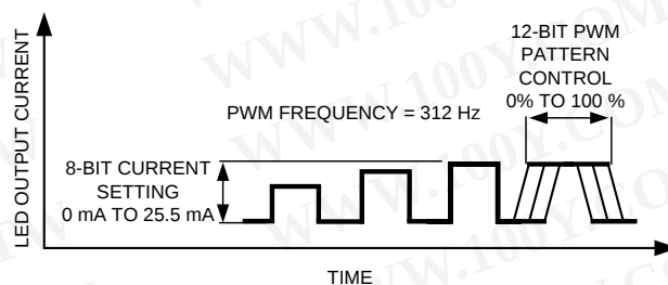
Figure 18. LED Pattern and Current Control Principle
