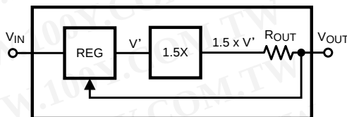
Figure 16. Charge Pump Output Resistance Model
