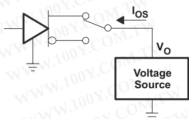
Figure 14. Driver Short-Circuit
