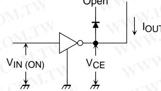
5. V_{IN} (ON)
