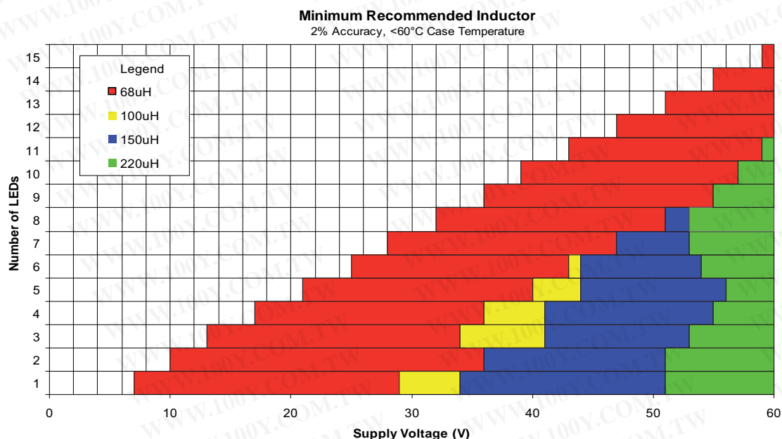
Figure 3 ZXLD1356 Minimum recommended inductor (TSOT)
