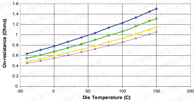
Lx on-resistance vs die temperature
