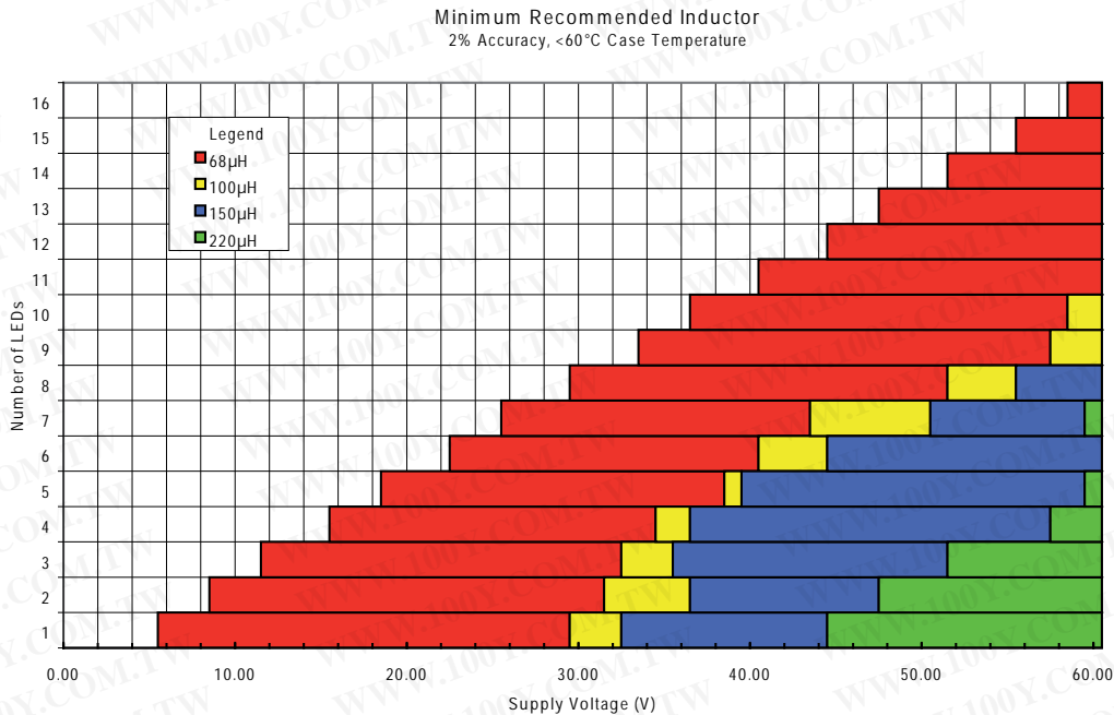
Figure 4 ZXLD1356 Minimum recommended inductor (DFN)
