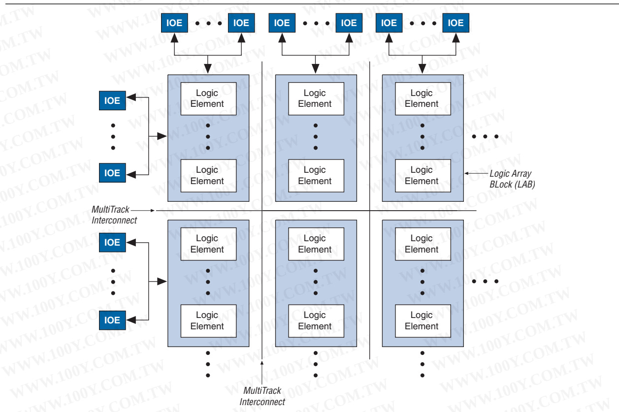
Figure 2-1. Device Block Diagram
