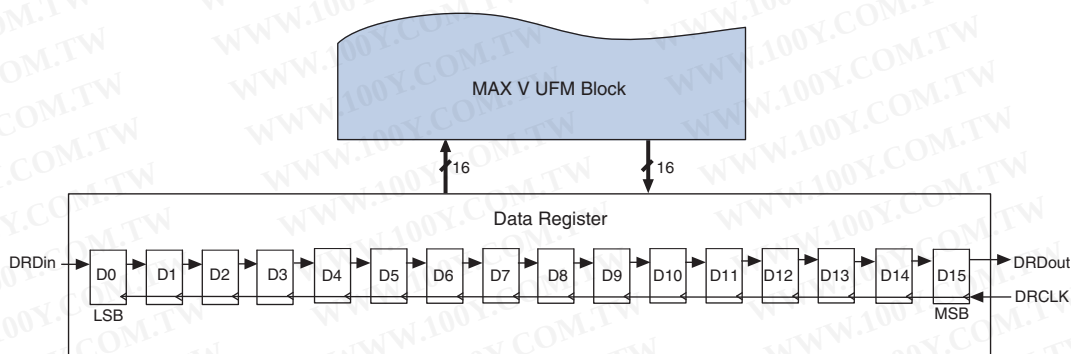
Figure 7-3. UFM Data Register
