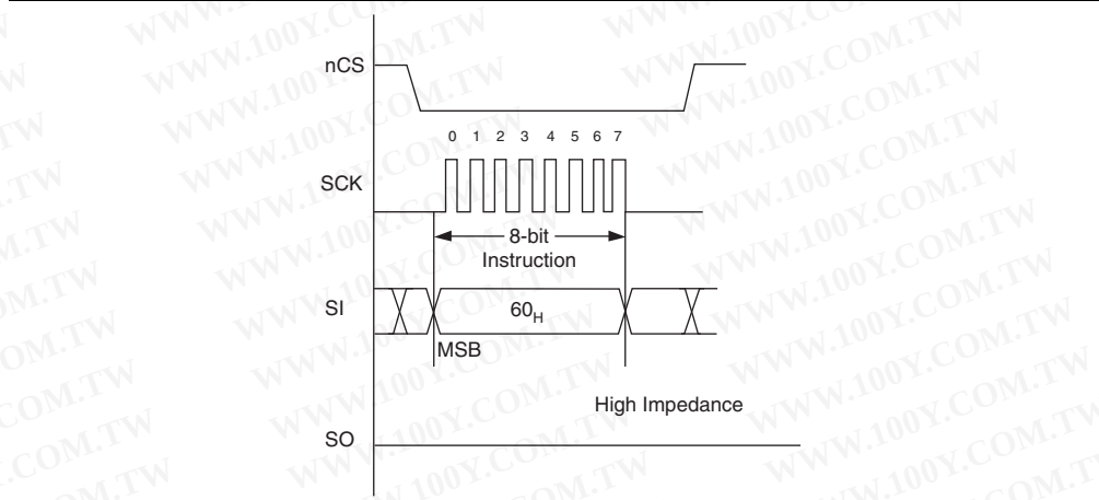
Figure 7-27. UFM-ERASE Operation Sequence
