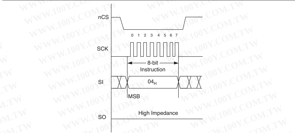
Figure 7-29. WRDI Operation Sequence
