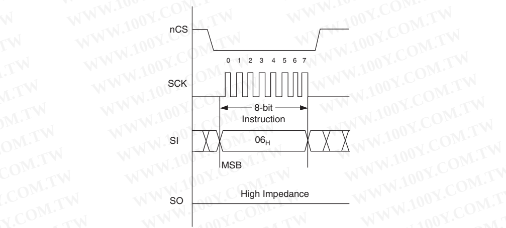
Figure 7-28. WREN Operation Sequence
