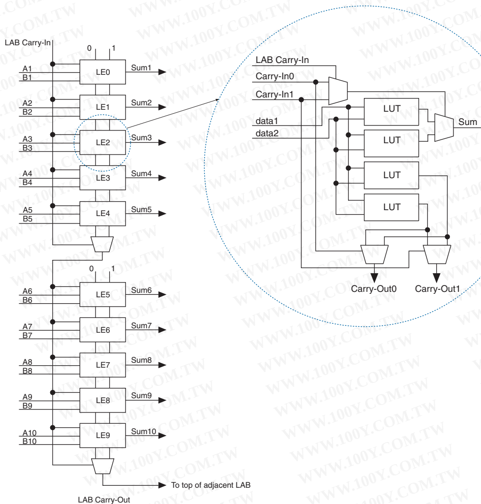
Figure 2-9. Carry-Select Chain
