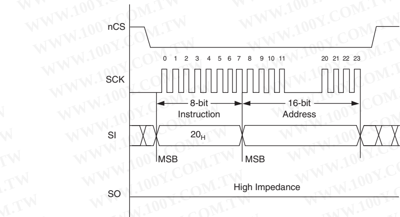
Figure 7-25. SECTOR-ERASE Operation Sequence for Extended Mode
