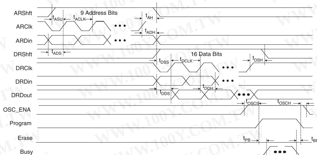
Figure 3-4. UFM Program Waveform
