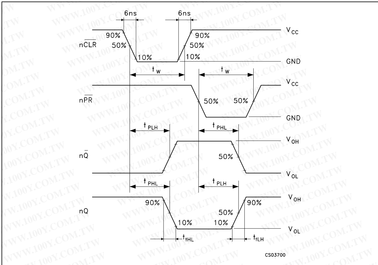
WAVEFORM 3 : MINIMUM PULSE WIDTH ( \overline{nCLR} and \overline{nPR} ), MINIMUM REMOVAL TIME ( \overline{nCLR} and nPR TO nCK ) ( f=1\text{MHz} ; 50% duty cycle)
