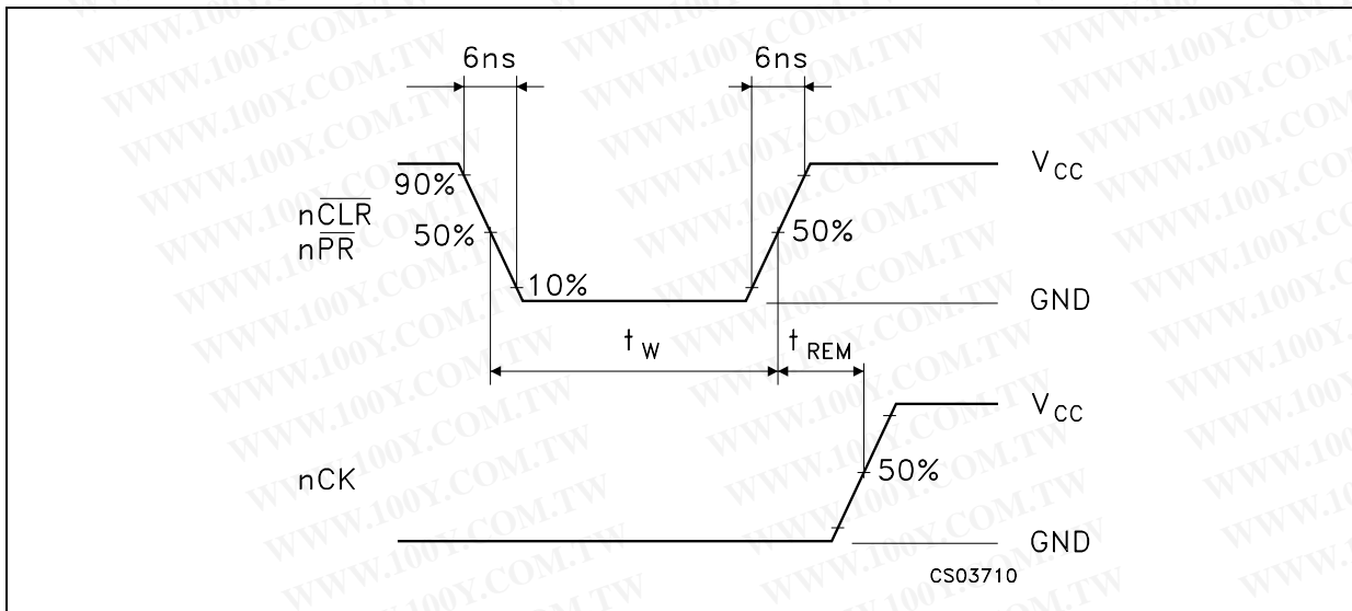
WAVEFORM 3 : MINIMUM PULSE WIDTH ( \overline{nCLR} and \overline{nPR} ), MINIMUM REMOVAL TIME ( \overline{nCLR} and nPR TO nCK ) ( f=1\text{MHz} ; 50% duty cycle)
