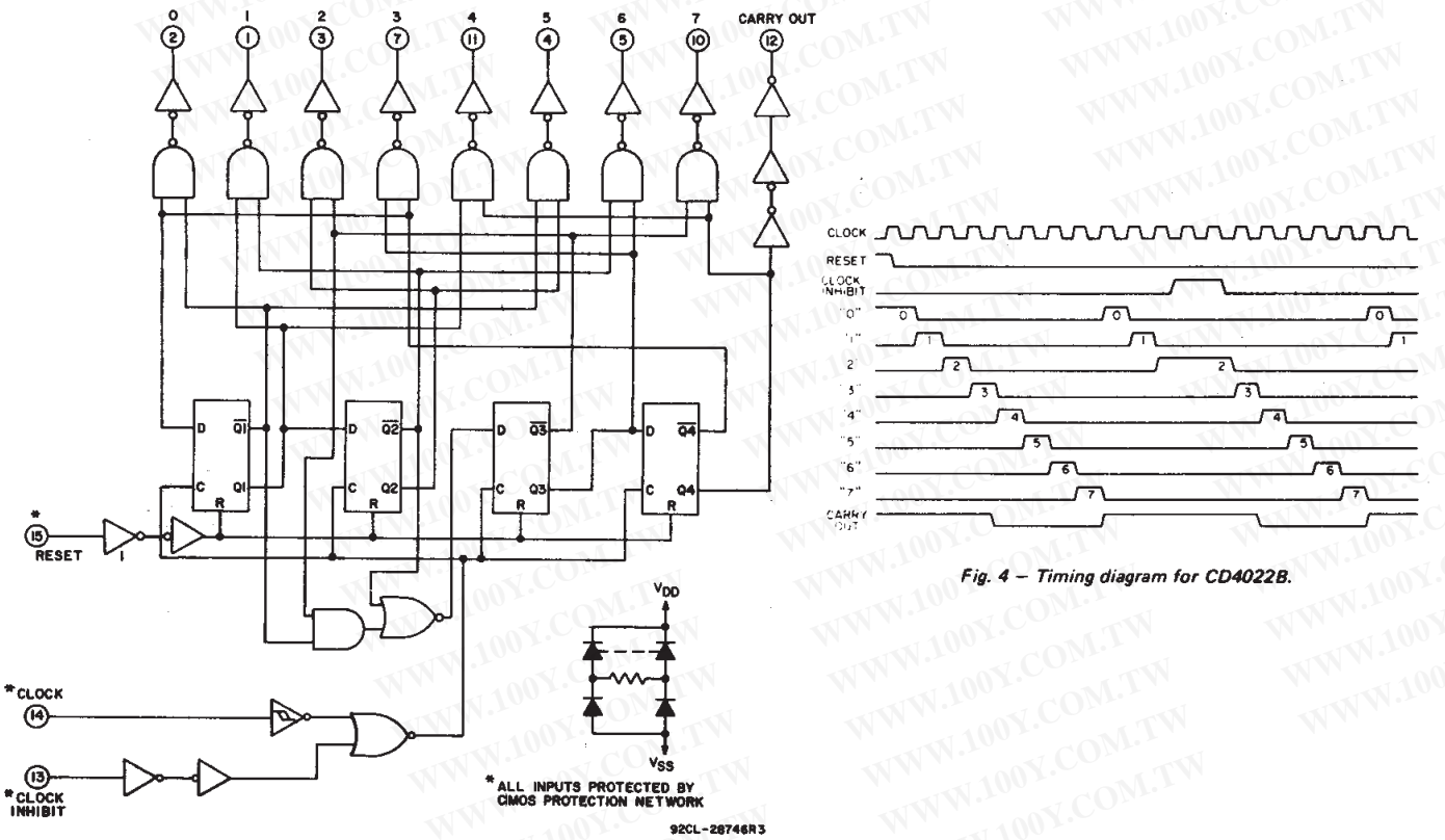
Fig. 3 - Logic diagram for CD4022B.
