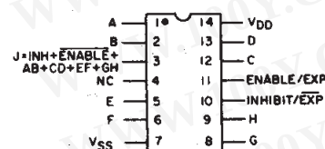
Top View TERMINAL ASSIGNMENT
