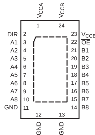
RHL PACKAGE (TOP VIEW)
