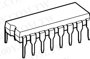
DIP16-P-300-2.54A
