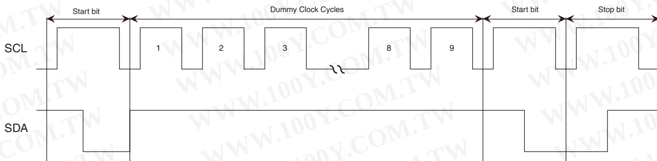
Figure 4-1. Software Reset
