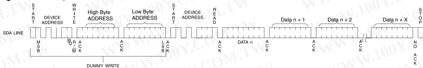
Figure 7-6. Sequential Read
