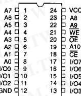
CERDIP, PDIP, SOIC Top View
