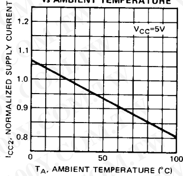
Fig. 6 – SUPPLY CURRENT (ACTIVE) vs AMBIENT TEMPERATURE
