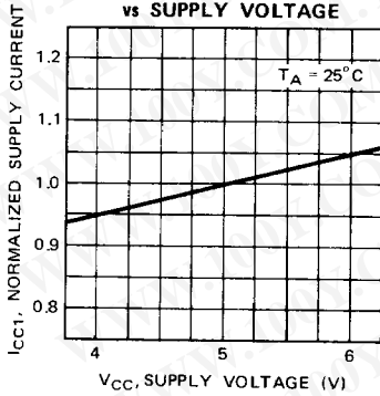
Fig. 5 – SUPPLY CURRENT (ACTIVE) vs SUPPLY VOLTAGE
