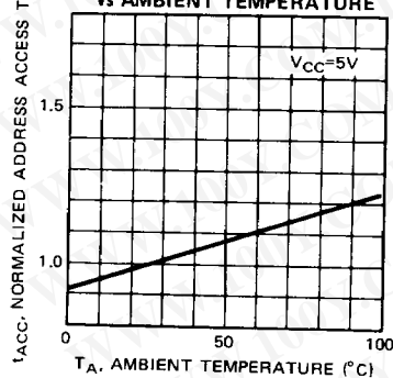
Fig. 8 – ADDRESS ACCESS TIME vs AMBIENT TEMPERATURE
