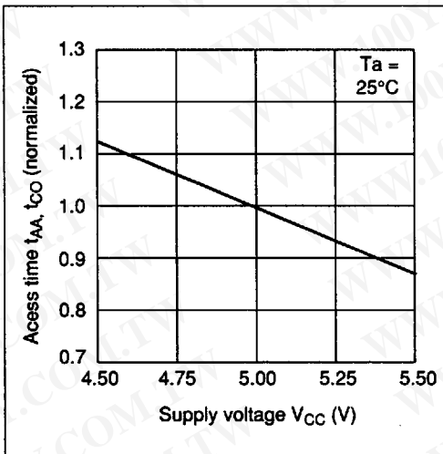
Access Time vs. Supply Voltage
