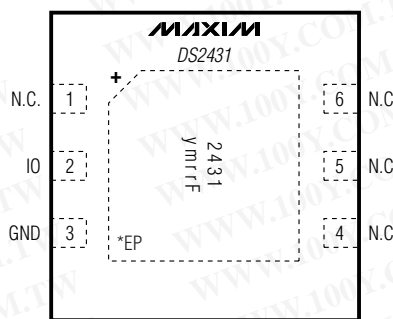
TDFN (3mm × 3mm)
