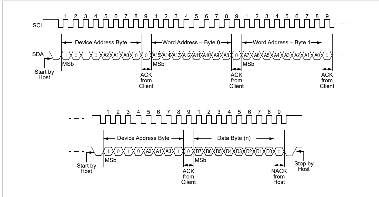
FIGURE 7-2: RANDOM READ
