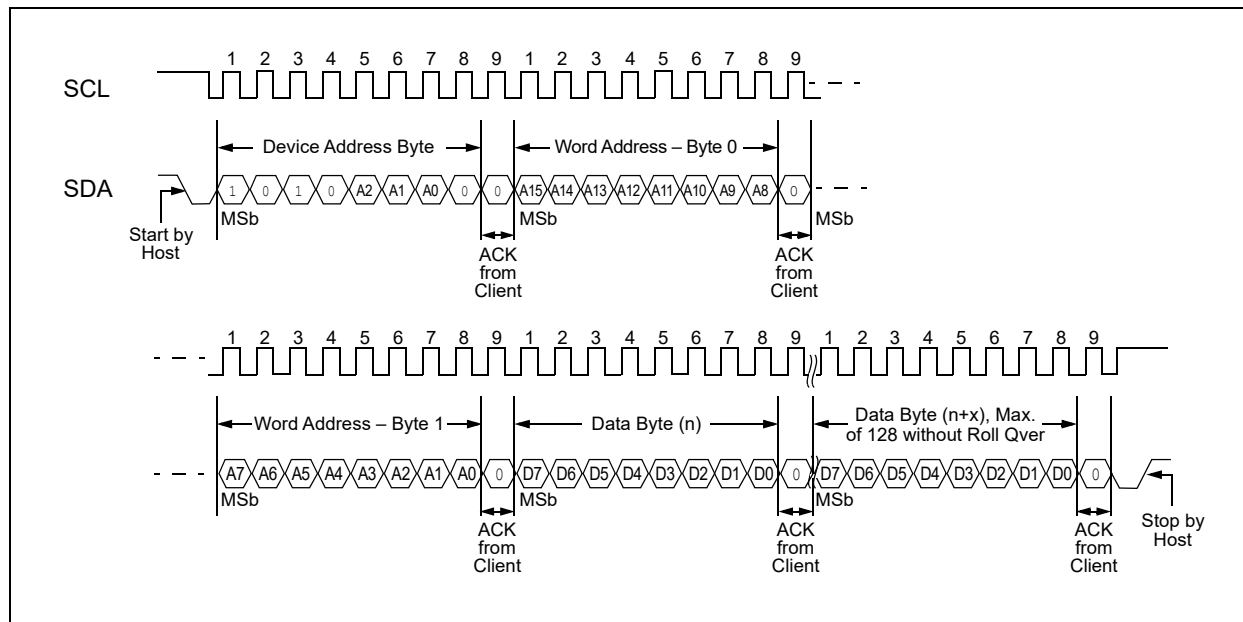
FIGURE 6-2: PAGE WRITE
