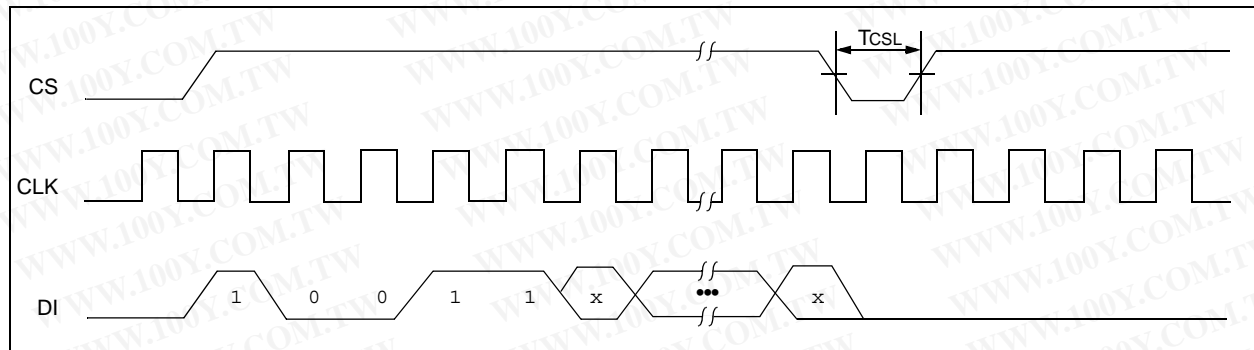
FIGURE 2-6: EWEN TIMING
