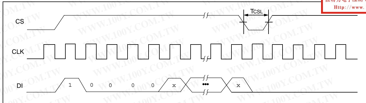
FIGURE 2-5: EWDS TIMING
