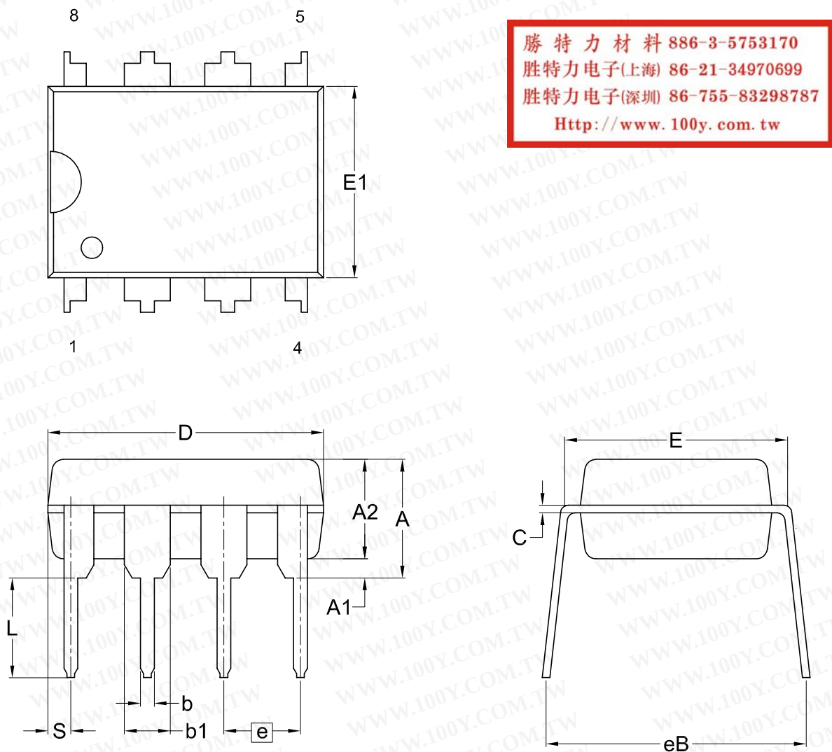
Title: Package Outline for PDIP 8L (300MIL)
