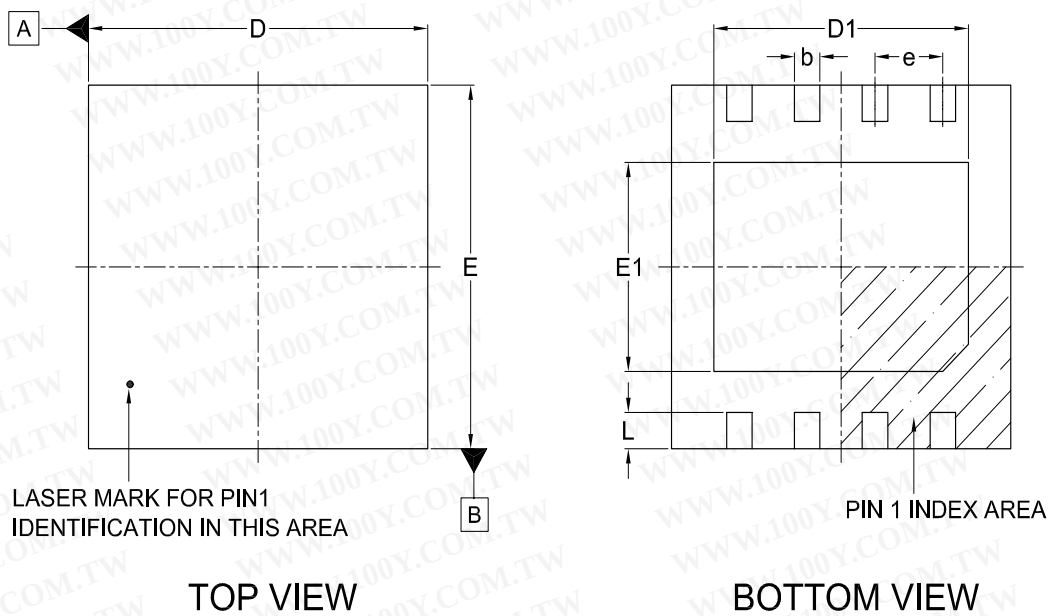
Title: Package Outline for USON 8L (4x4x0.6MM, LEAD PITCH 0.8MM)
