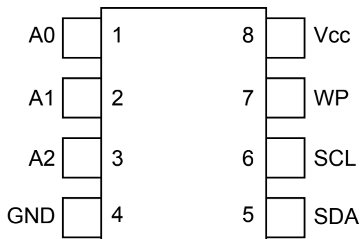
8-lead SOIC/TSSOP
