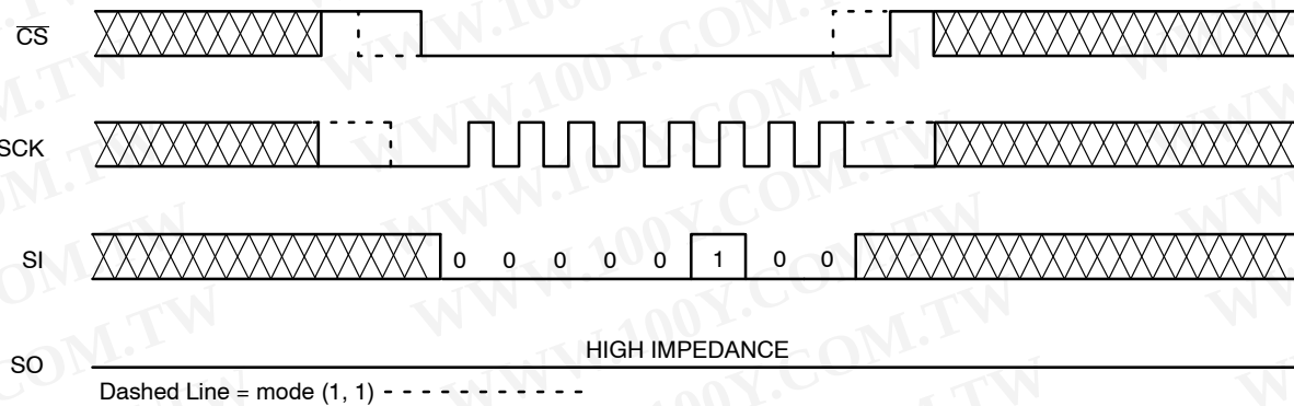
Figure 4. WRDI Timing
