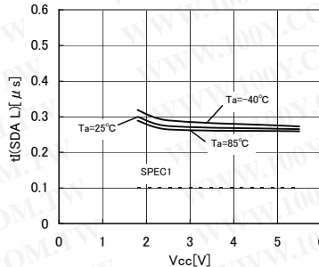
Fig.32 Noise removal valid time t(SDA L)
