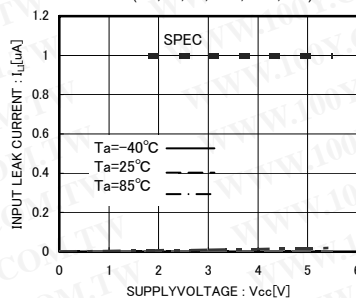
Fig.7 Input leak current I_I (A0,A2,SCL,WP)
