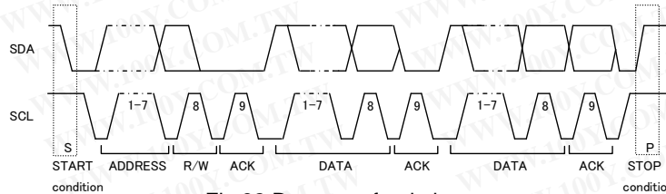
Fig.32 Data transfer timing
