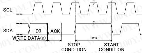
Fig.1-(a) Sync data input / output timing
