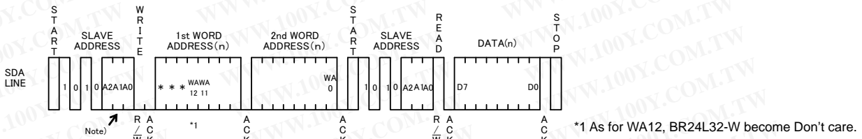
Fig.44 Random read cycle (BR24L32/64 -W)
