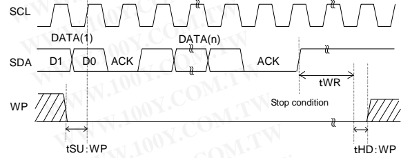
Fig.1-(d) WP timing at write execution
