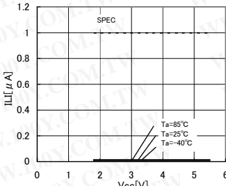
Fig.7 Input leak current IIL1 (SCL,WP)
