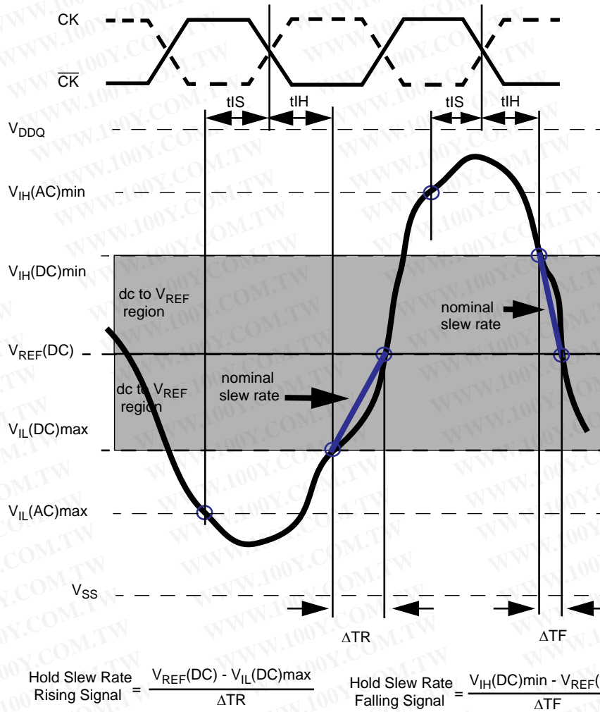
Figure 17. Illustration of nominal slew rate for tIH
