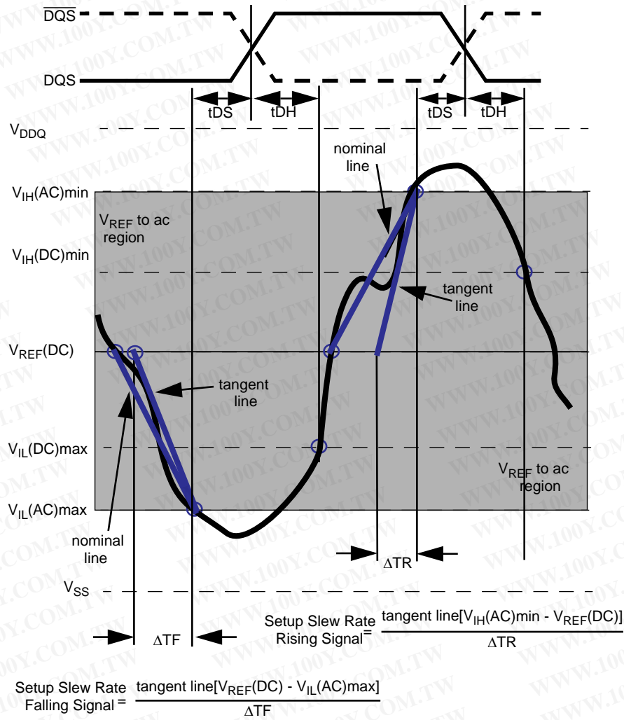
Figure 9. Illustration of tangent line for tDS (differential DQS, DQS-bar)
