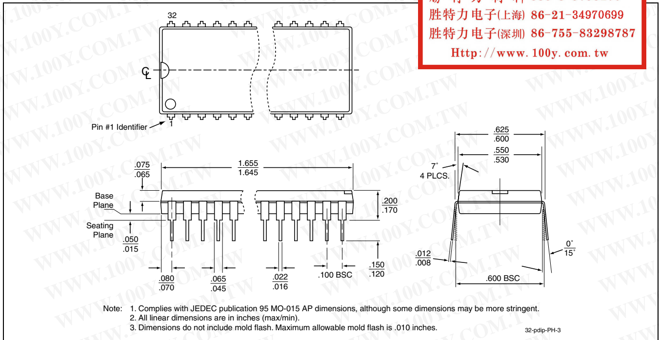
32-PIN PLASTIC DUAL IN-LINE PINS (PDIP) SST PACKAGE CODE: PH
