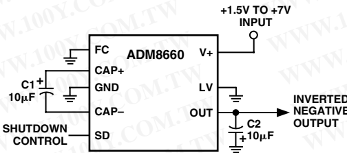
Figure 6. ADM8660 Voltage Inverter Configuration
