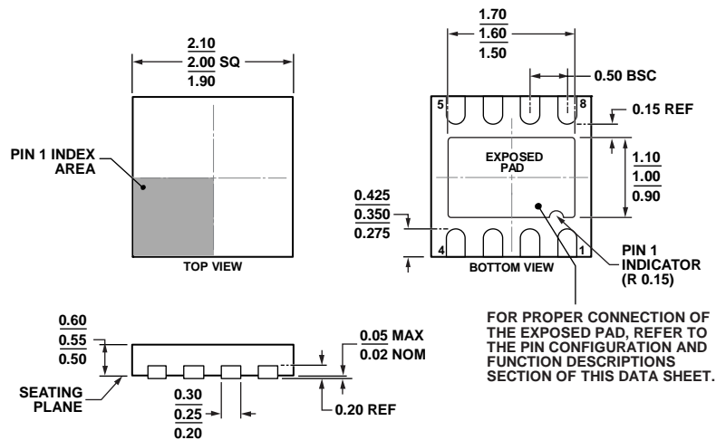
Figure 46. 8-Lead Lead Frame Chip Scale Package [LFCSF_UD]
