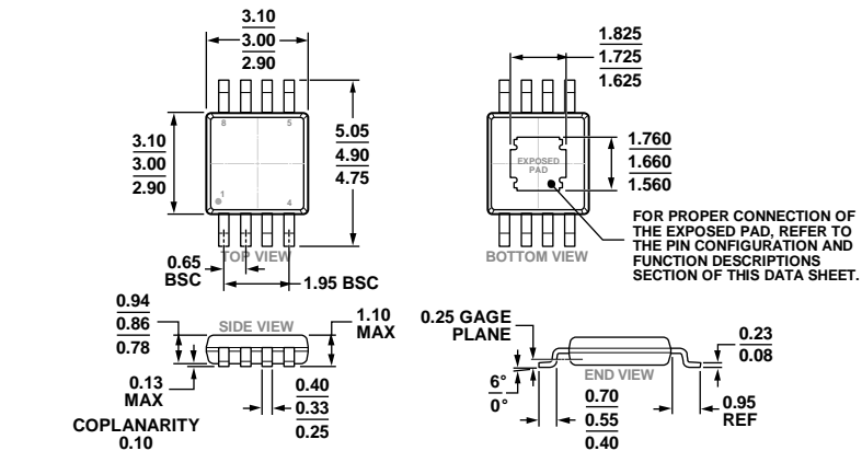
Figure 45. 8-Lead Mini Small Outline Package with Exposed Pad [MINI_SO_EP] (RH-8-1)
