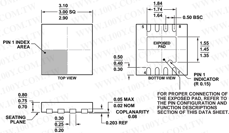
Figure 44. 8-Lead Frame Chip Scale Package [LFCSF] 3 mm x 3 mm Body and 0.75 mm Package Height (CP-8-13) Dimensions shown in millimeters
