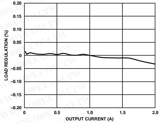
Figure 13. ADP2302 Load Regulation, V_{OUT} = 3.3V , V_{IN} = 12V
