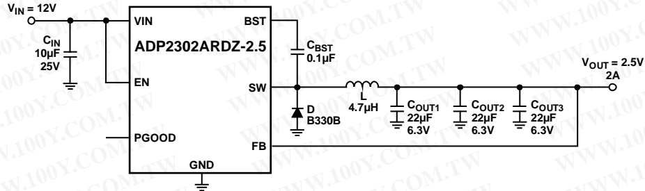
Figure 56. ADP2302 Typical Application, V_{IN} = 12V , V_{OUT} = 2.5V , 2A
