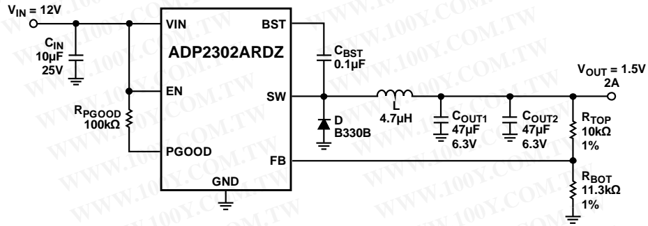
Figure 54. ADP2302 Typical Application, V_{IN} = 12V , V_{OUT} = 1.5V , 2A
