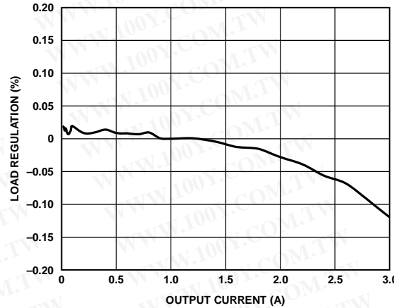
Figure 14. ADP2303 Load Regulation, V_{OUT} = 3.3V , V_{IN} = 12V
