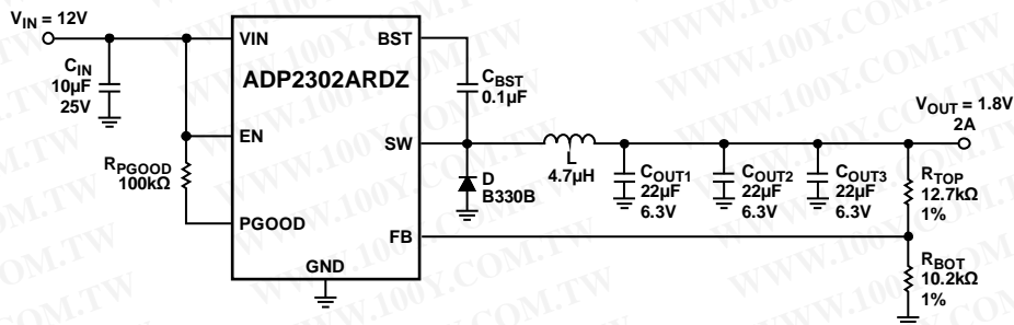
Figure 55. ADP2302 Typical Application, V_{IN} = 12V , V_{OUT} = 1.8V , 2A
