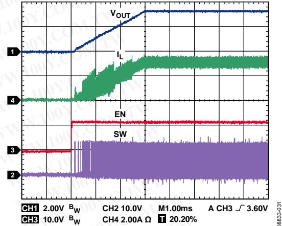
Figure 31. Soft Start with Full Load, V_{OUT} = 3.3V , V_{IN} = 12V
