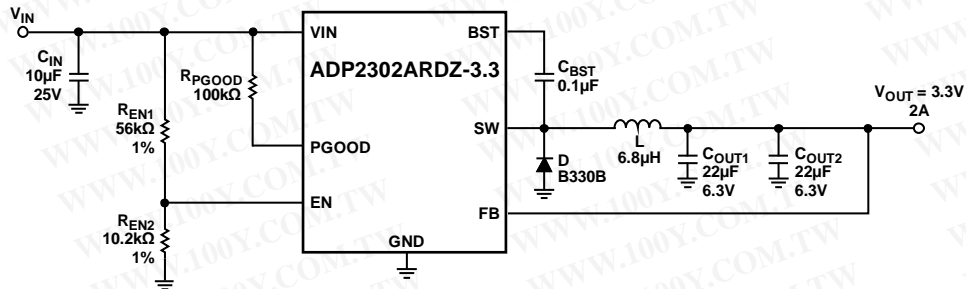
Figure 57. ADP2302 Typical Application, V_{IN} = 12V , V_{OUT} = 3.3V , 2A, with Programmable 7.8V UVLO
