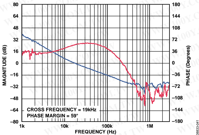
Figure 41. ADP2303 Bode Plot, V_{OUT} = 3.3V , V_{IN} = 12V , L = 4.7\mu H , C_{OUT} = 2 \times 47\mu F
