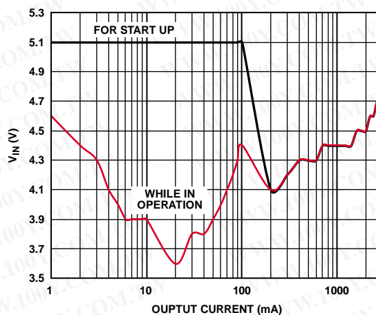
Figure 46. Minimum Input Voltage vs. Load Current
