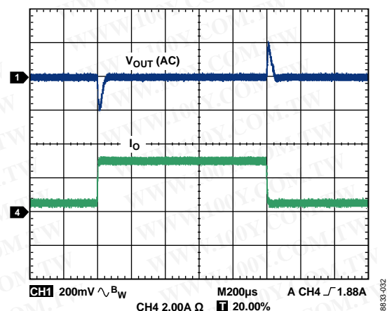
Figure 32. ADP2303 Load Transient, 0.5 A to 3.0 A, V_{OUT} = 3.3V , V_{IN} = 12V , L = 4.7\mu H , C_{OUT} = 2 \times 47\mu F
