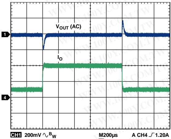
Figure 30. ADP2302 Load Transient, 0.5 A to 2.0 A, V_{OUT} = 5.0V , V_{IN} = 12V , L = 6.8\mu H , C_{OUT} = 2 \times 22\mu F
