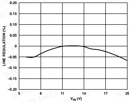
Figure 11. ADP2303 Line Regulation, V_{OUT} = 3.3V , I_{OUT} = 3A
