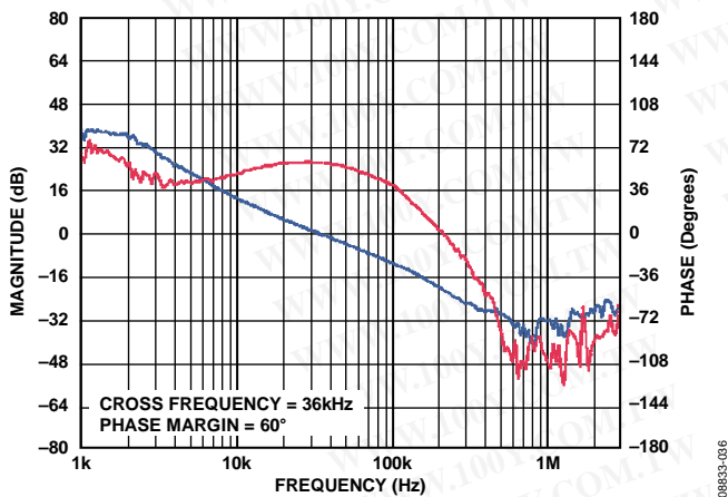
Figure 36. ADP2302 Bode Plot, V_{OUT} = 2.5\text{ V} , V_{IN} = 12\text{ V} , L = 4.7\ \mu\text{H} , C_{OUT} = 3 \times 22\ \mu\text{F}
