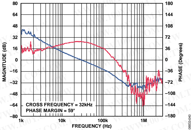
Figure 40. ADP2302 Bode Plot, V_{OUT} = 5V , V_{IN} = 12V , L = 6.8\mu H , C_{OUT} = 2 \times 22\mu F
