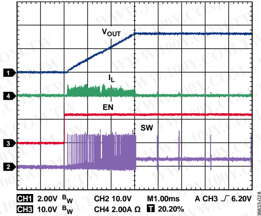
Figure 28. Soft Start Without Load, V_{OUT} = 3.3V , V_{IN} = 12V
