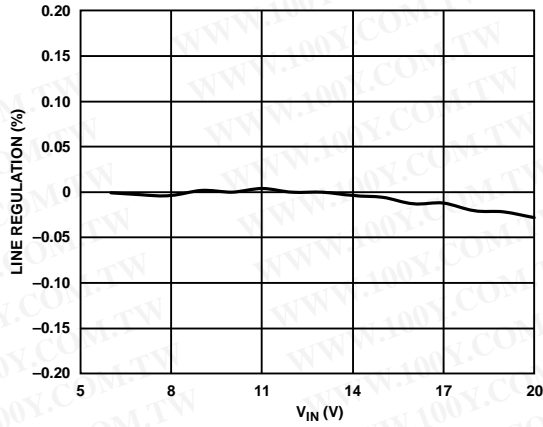
Figure 10. ADP2302 Line Regulation, V_{OUT} = 3.3V , I_{OUT} = 2A
