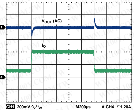
Figure 33. ADP2302 Load Transient, 0.5 A to 2.0 A, V_{OUT} = 3.3V , V_{IN} = 12V , L = 6.8\mu H , C_{OUT} = 2 \times 22\mu F
